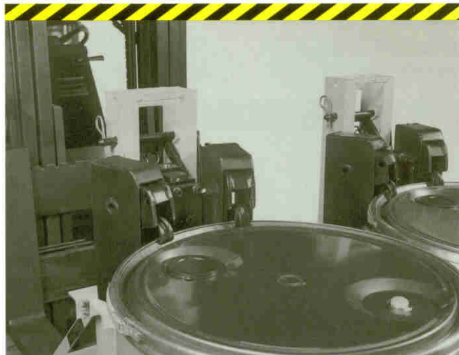
Double "Parrot-Beak"™ clamps assure safe, dependable handling on all standard steel, plastic and fibre drums.
